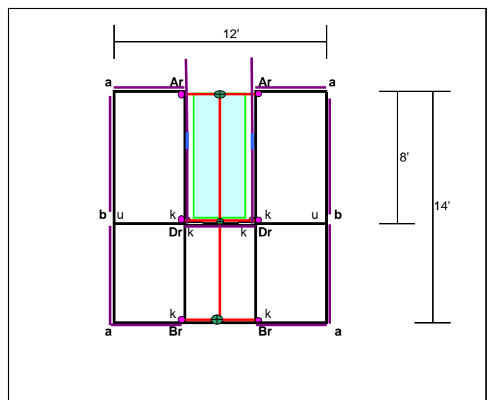
Paddle-Safe Adaptive Kayak Dock System - Design #4A
