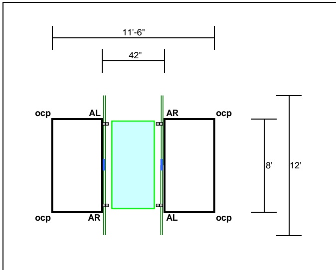
Paddle-Safe Kayak Dock System - Design #1
